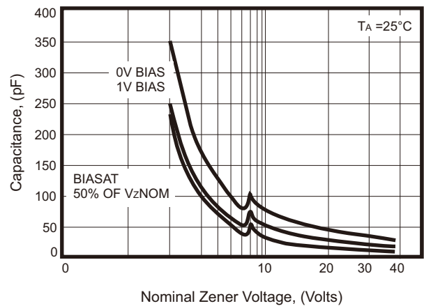
Fig.6 - Typical Capacitance
