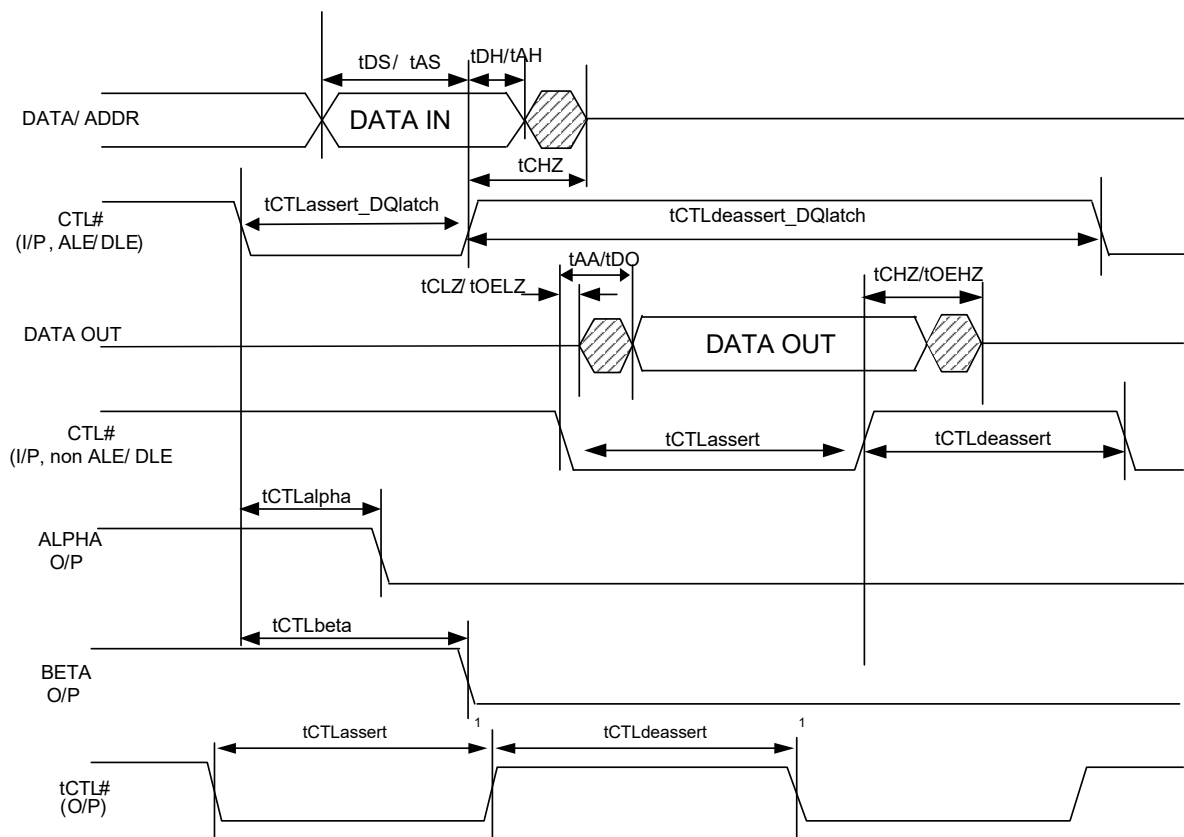
Figure 9. GPIF II Timing in Asynchronous Mode
