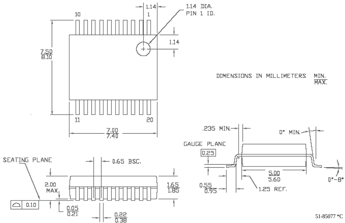
Figure 38: 20-Pin Shrink Small Outline Package O20
