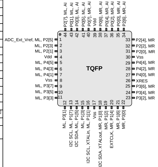
Figure 4. Pin Diagram
