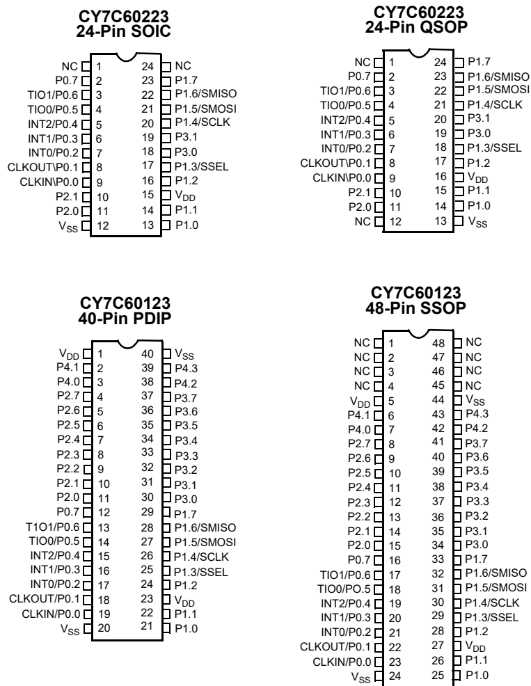
Figure 7-1. Package Configurations
