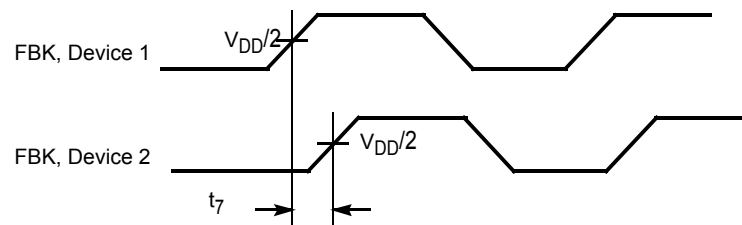
Figure 7. Device-Device Skew
