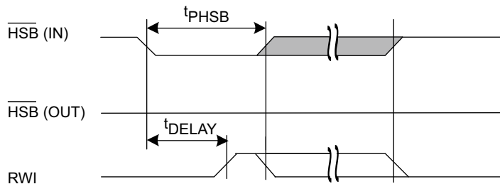
Figure 22. Soft Sequence Processing [62, 63]
