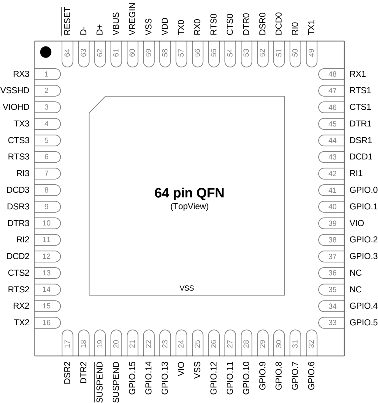
Figure 2. QFN-64 Pinout
