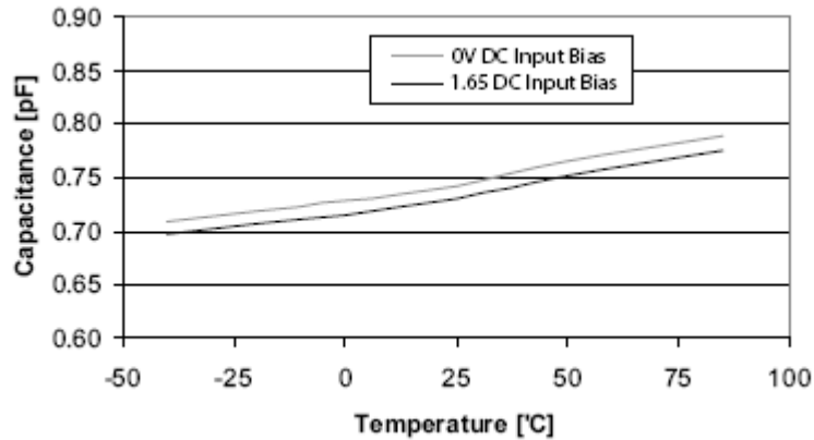
Figure 2. Typical Variation of C_{IN} vs. Temp ( f = 1 MHz, V_{IN} = 30 mV, V_P = 3.3 V, V_N = 0 V, 0.1 \mu\text{F} chip capacitor between V_P and V_N )
