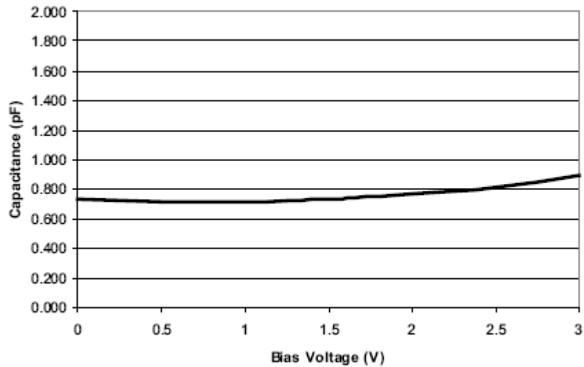
Figure 1. Typical Variation of C_{IN} vs. V_{IN} ( f = 1 MHz, V_P = 3.3 V, V_N = 0 V, 0.1 \mu\text{F} chip capacitor between V_P and V_N , T_A = 25^\circ\text{C} )
