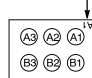
CM1230-04 6-bump CSP Package
