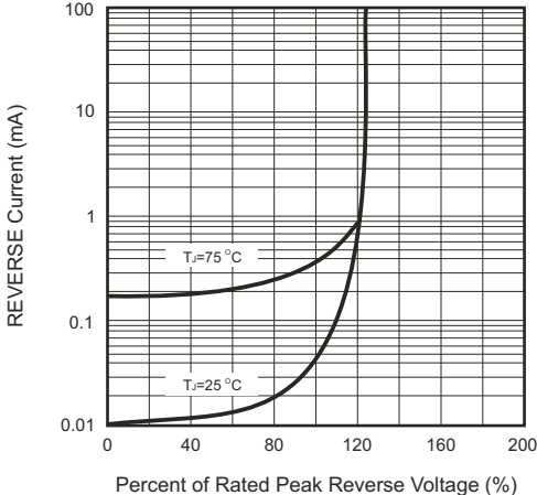
Fig.4- Reverse Characteristics
