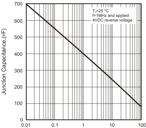
Fig.5- Junction Capacitance
