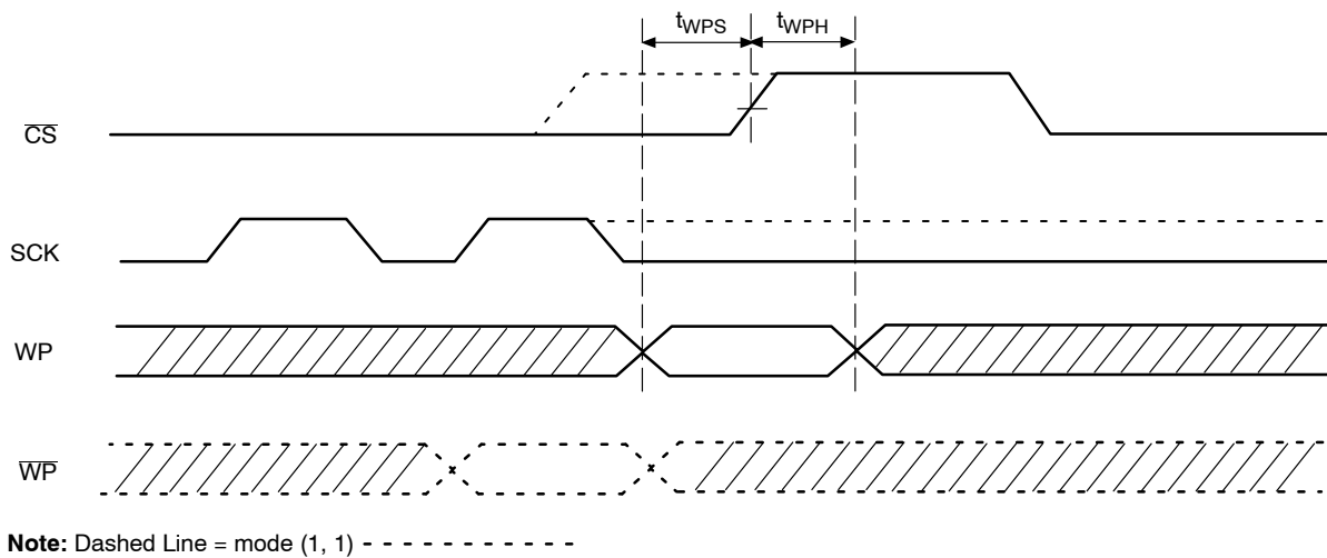
Figure 8. \overline{WP} Timing
