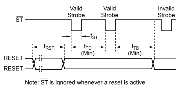
Figure 7. Timing Diagram: Strobe Input
