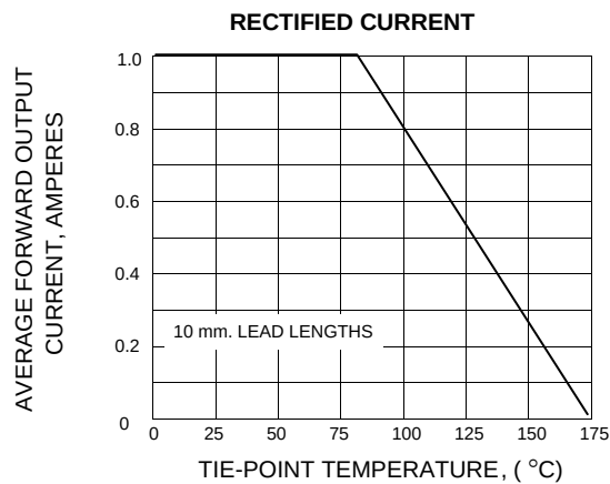
FIG.2 - DERATING CURVE FOR OUTPUT
