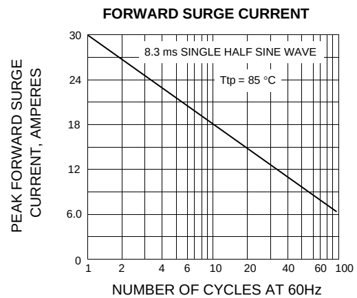
FIG.3 - MAXIMUM NON-REPETITIVE PEAK
