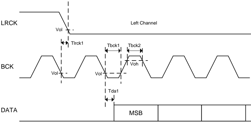
Figure 19 Timing chart
