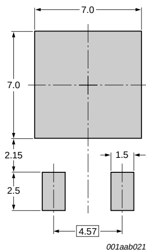
Fig 14. SOT428: minimum pad size for surface-mounting
