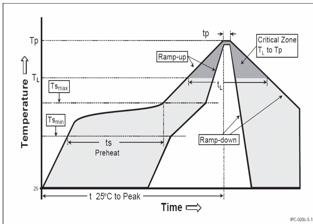
Figure 45: Soldering profile
