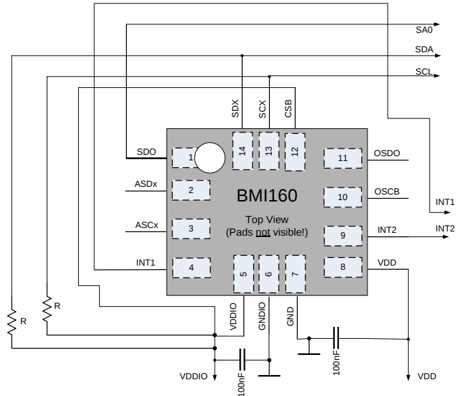
Figure 33: Only I2C as primary interface
