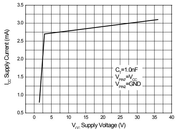
Standard Supply Current vs. Supply Voltage
