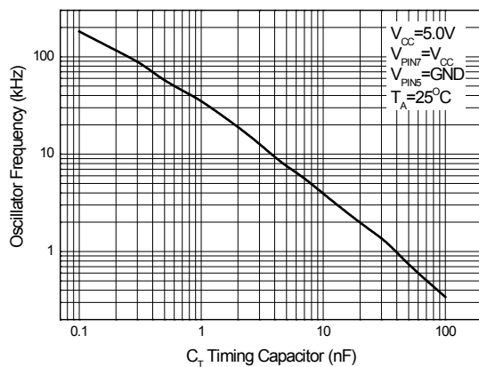
Oscillator Frequency vs. Timing Capacitor
