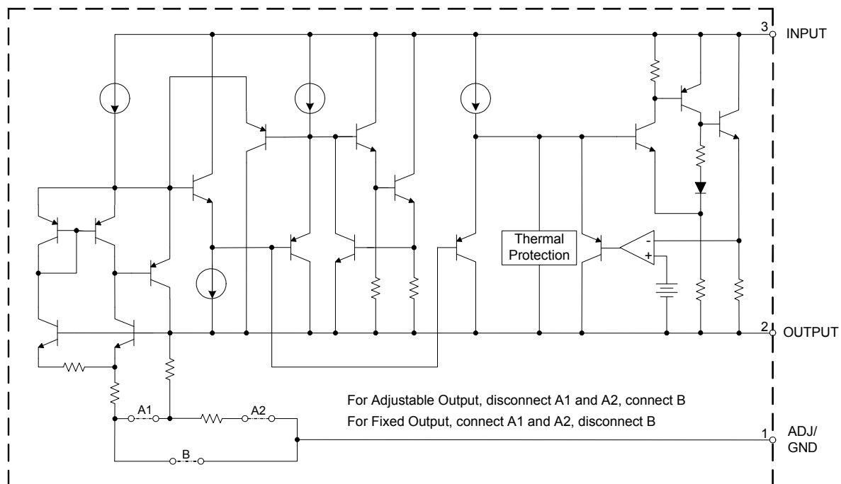
Figure 3. Functional Block Diagram of AZ1084C
