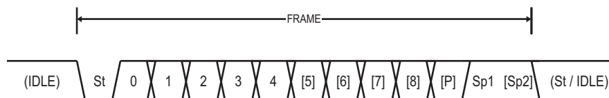
Figure 56. Frame Formats
