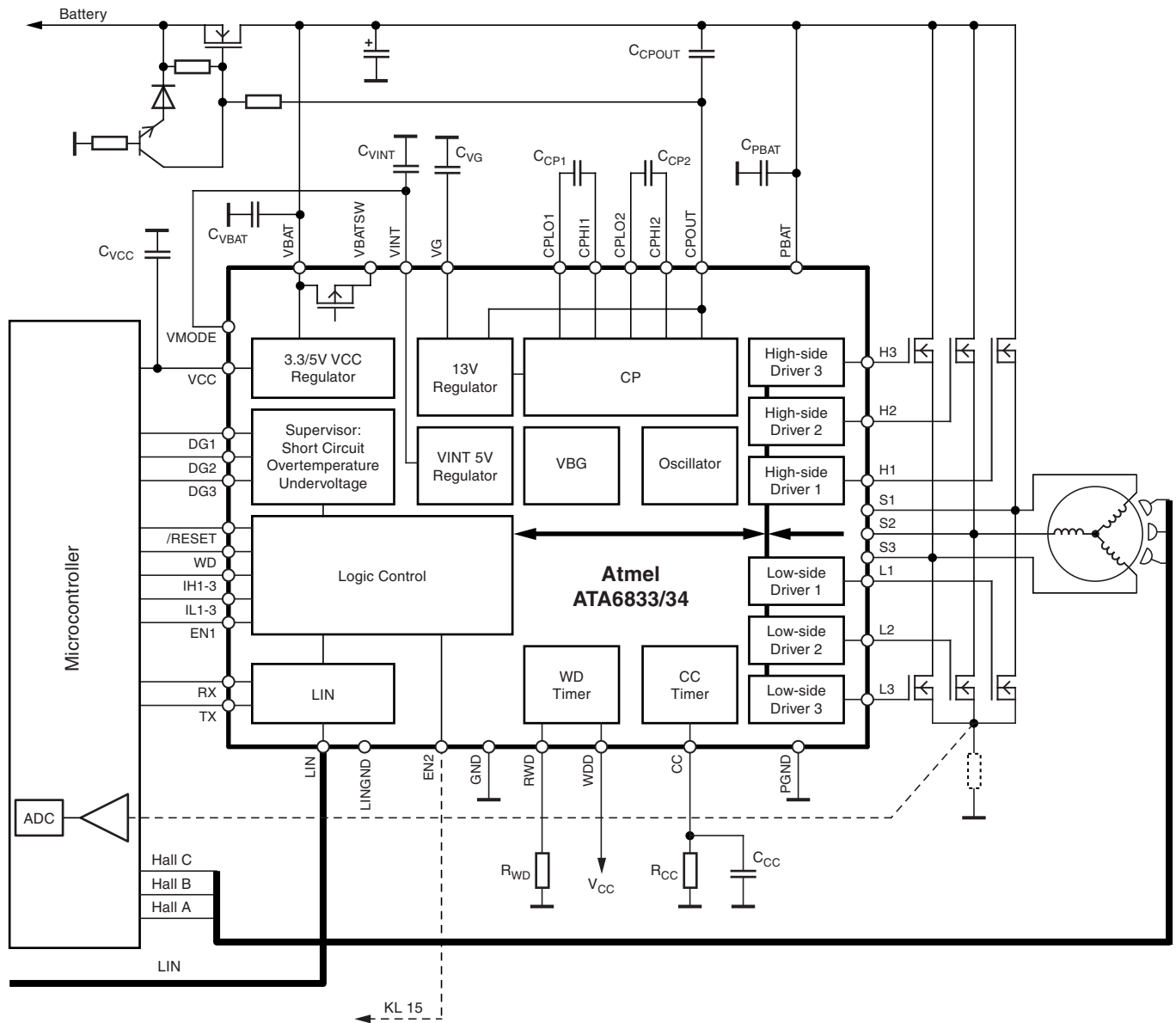
Figure 9-1. Typical Application
