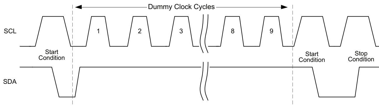
Figure 7-4. Software reset
