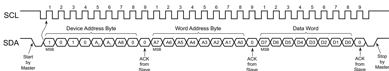
Figure 5-1. Byte Write
