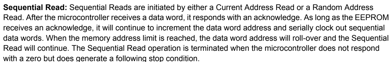
Figure 9-3. Sequential Read
