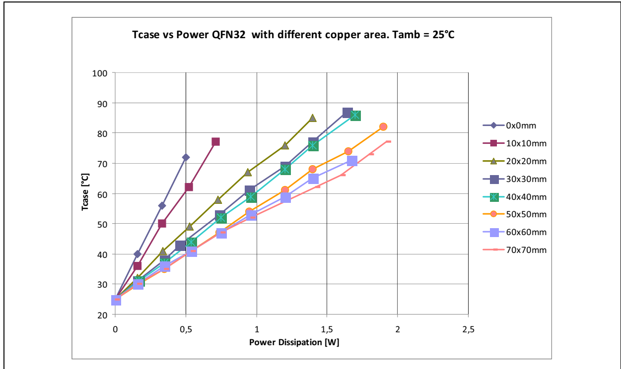
Figure 10: TCASE vs. Power with Different Copper Area @ T_{AMB} = 25^{\circ}\text{C}
