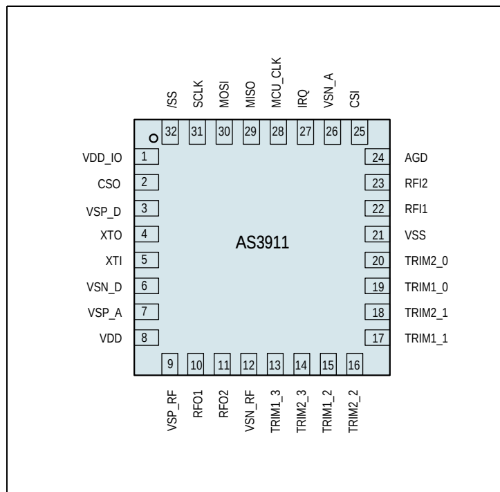
Figure 3: Pin Diagram
