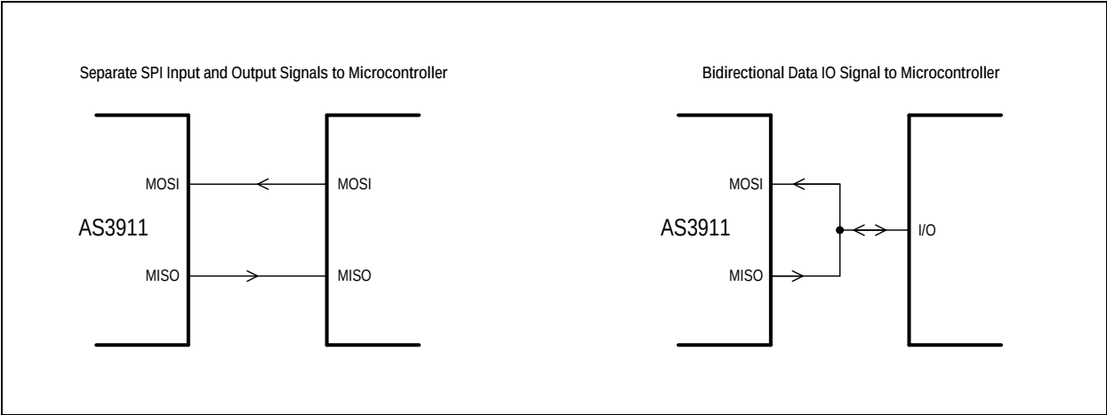
Figure 24: Signal to Microcontroller
