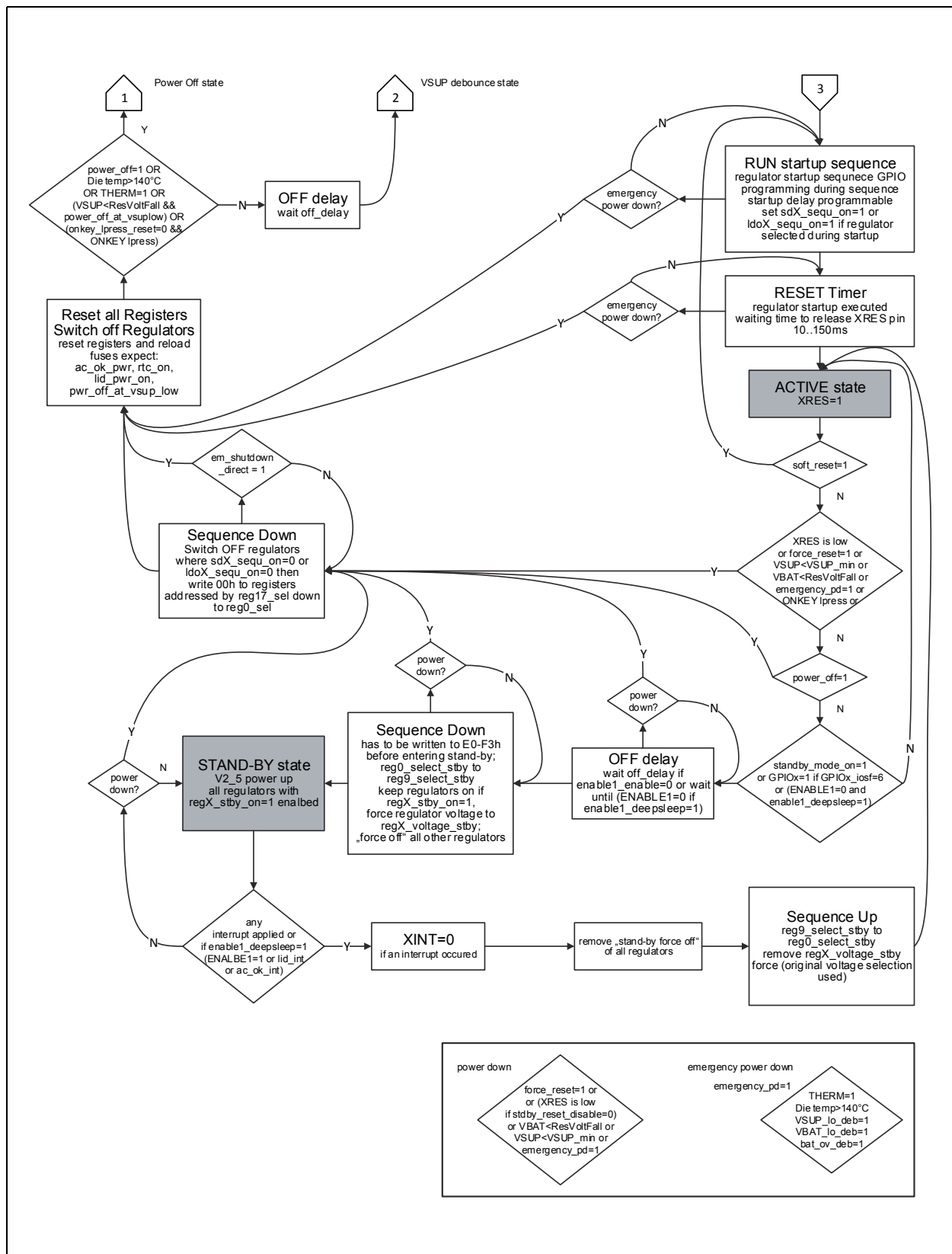
Figure 49: Start-Up Flow Chart 2/2
