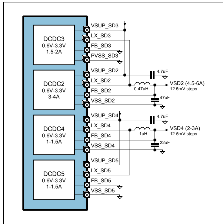
Figure 19: DC/DC Buck Converter SD2+SD3 & SD4+SD5 Mode
