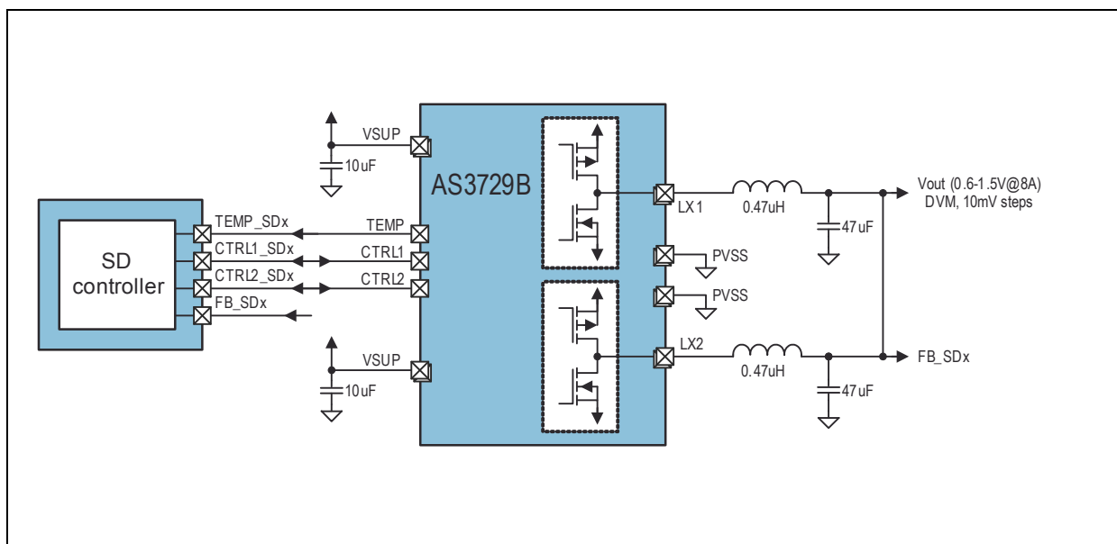
Figure 23: SD1 DC/DC Buck Controller 8A Peak Block Diagram
