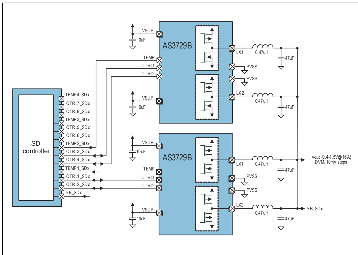
Figure 26: SD0 DC/DC Buck Controller 16A Block Diagram
