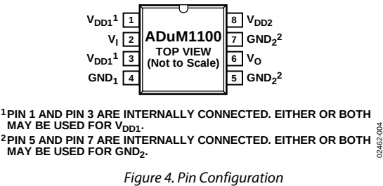
Figure 4. Pin Configuration
