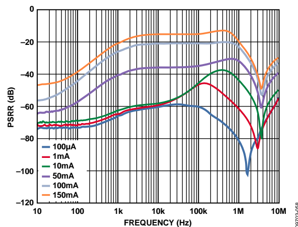
Figure 43. LDO PSRR Across Output Load, V_{IN3} = 3.3\text{ V} , V_{OUT3} = 3.0\text{ V}
