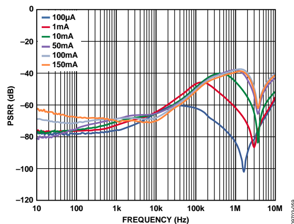
Figure 44. LDO PSRR Across Output Load, V_{IN3} = 5.0\text{ V} , V_{OUT3} = 2.8\text{ V}
