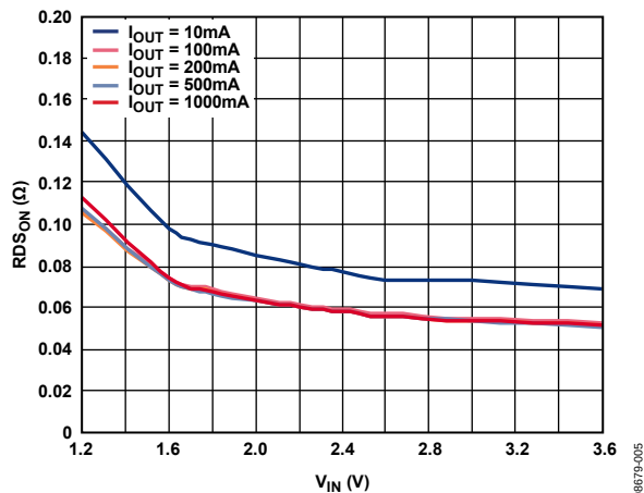
Figure 7. R_{DS(on)} vs. Input Voltage ( V_{IN} ), WLCSP
