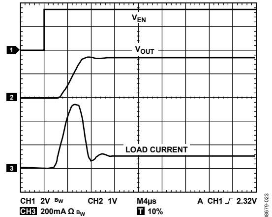
Figure 28. Typical Rise Time and Inrush Current, C_{LOAD} = 1\text{ }\mu\text{F} , V_{IN} = 1.8\text{ V} , Load = 200 mA
