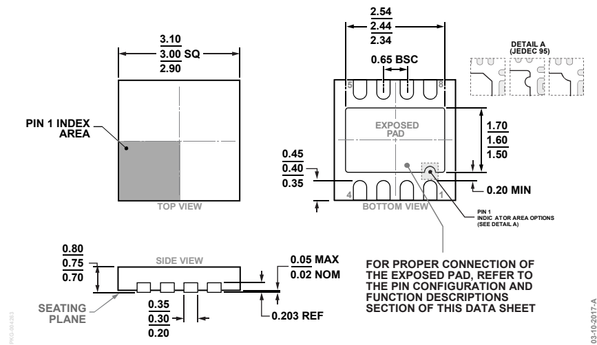
Figure 28. 8-Lead Lead Frame Chip Scale Package [LFCSP] 3 mm × 3 mm Body and 0.75 mm Package Height (CP-8-19) Dimensions shown in millimeters
