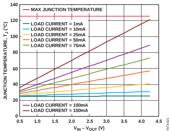
Figure 30. 500 mm 2 of PCB Copper, T_A = 25^\circ\text{C}
