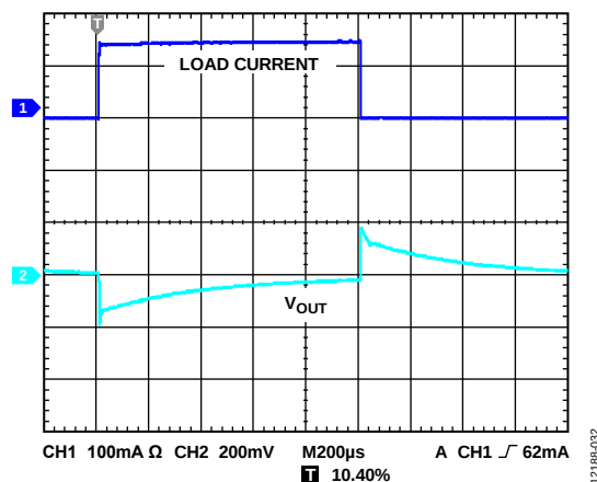
Figure 36. Output Transient Response, C_{OUT} = 1\text{ }\mu\text{F} , CH1 = Load Current, CH2 = V_{OUT}
