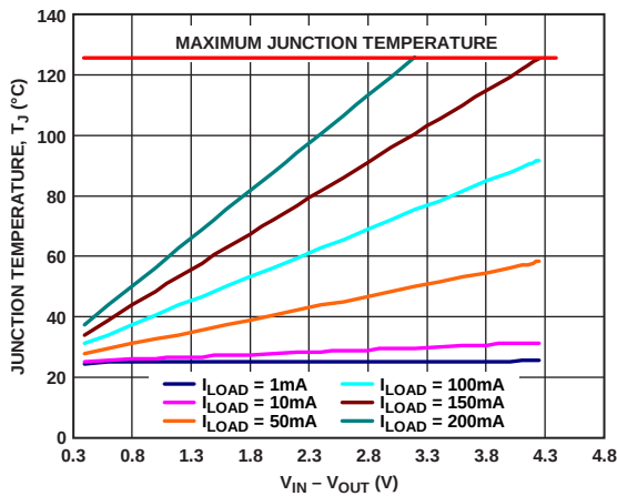
Figure 44. 100 mm 2 of PCB Copper, WLCSP, T_A = 25^\circ\text{C}
