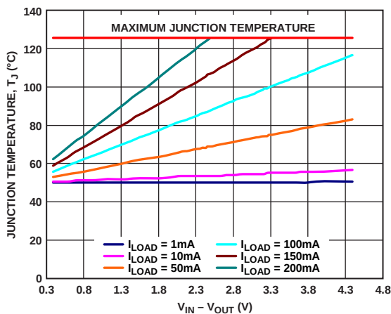
Figure 45. 500 mm 2 of PCB Copper, WLCSP, T_A = 50^\circ\text{C}
