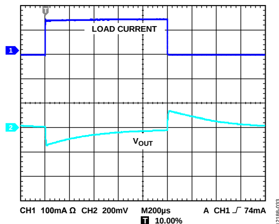
Figure 37. Output Transient Response, C_{OUT} = 10\text{ }\mu\text{F} , CH1 = Load Current, CH2 = V_{OUT}
