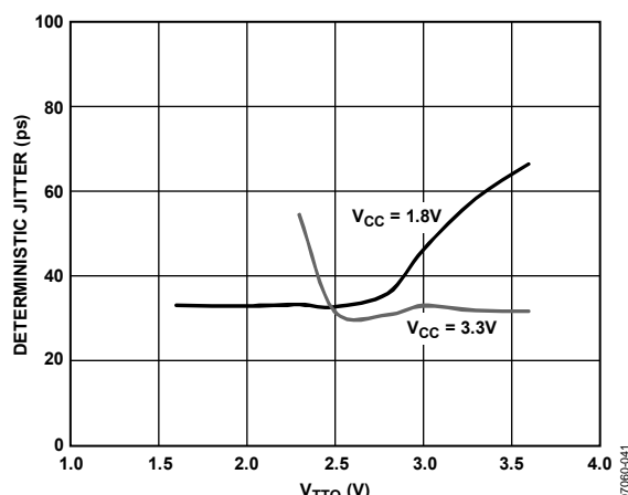
Figure 35. Deterministic Jitter vs. Output Termination Voltage ( V_{TT0} )
