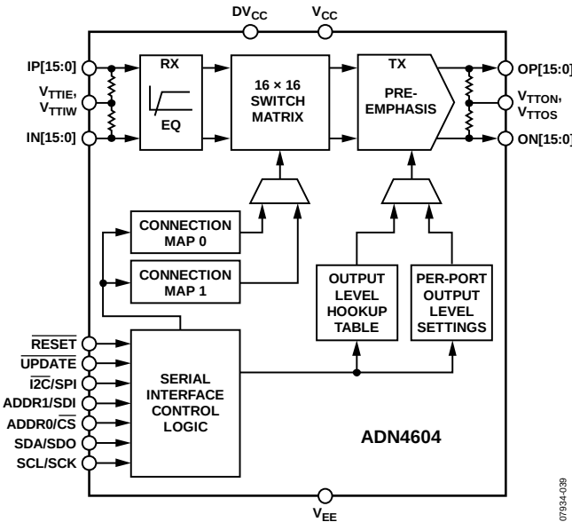
Figure 39. Block Diagram
