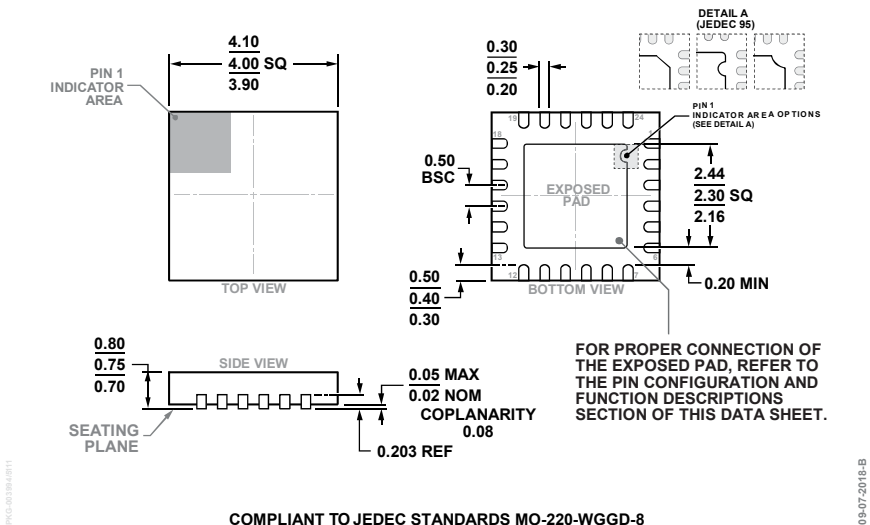
COMPLIANT TO JEDEC STANDARDS MO-220-WGGD-8 Figure 34. 24-Lead Lead Frame Chip Scale Package [LFCSP] 4 mm x 4 mm Body and 0.75 mm Package Height (CP-24-14) Dimensions shown in millimeters
