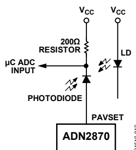
Figure 30. Single Measurement of I_{MPD} Across a Sense Resistor
