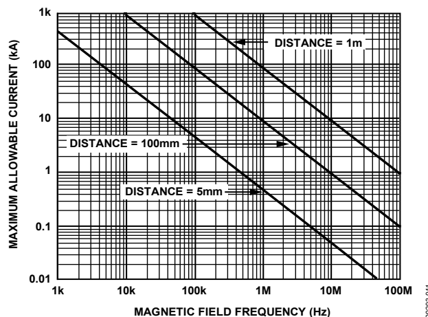
Figure 27. Maximum Allowable Current for Various Current-to-ADM3053 Spacings
