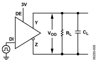
Figure 8. Driver Timing Test Circuit
