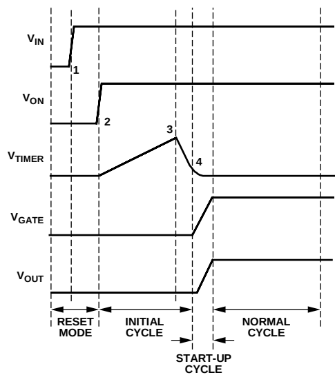
Figure 33. Power-Up Timing
