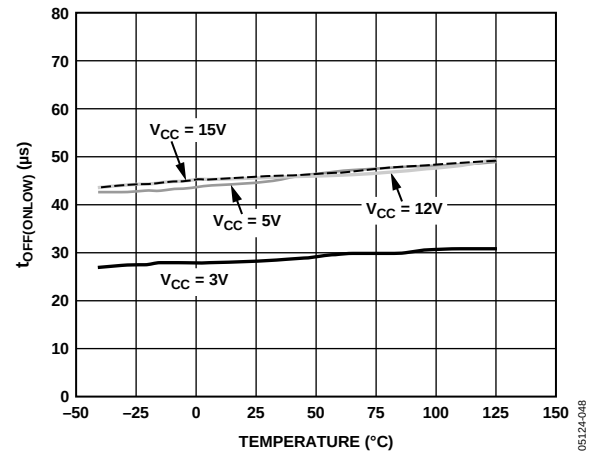
Figure 25. t_{\text{OFF}}(\text{ONLOW}) vs. Temperature
