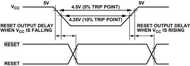
Figure 9. Reset Output Delay
