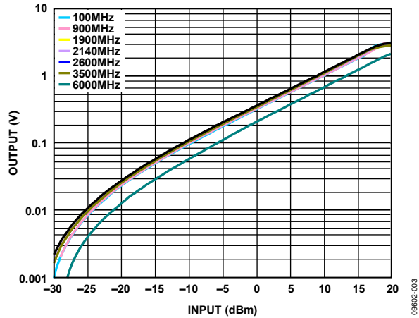
Figure 4. V_{\text{ENV}} - V_{\text{REF}} Output vs. Input Level, at Various Frequencies at 25^\circ\text{C} , Supply 5\text{ V}
