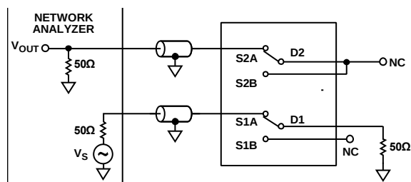
Figure 27. Off Isolation
