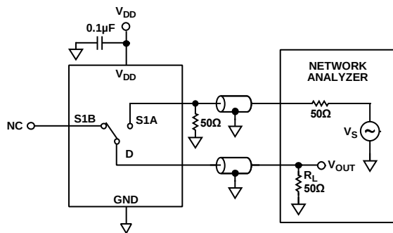
Figure 27. Off Isolation
