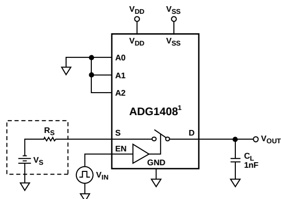
Figure 32. Charge Injection
