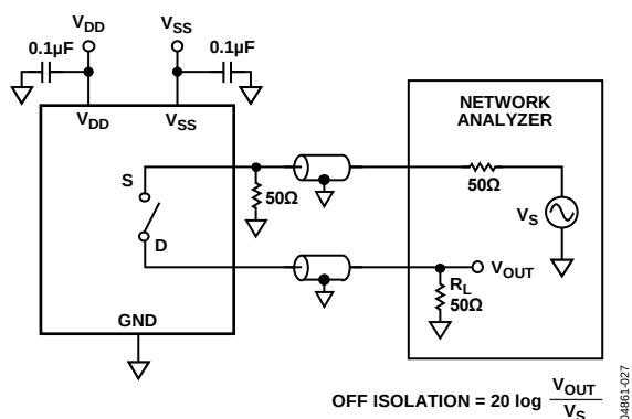
Figure 33. Off Isolation
