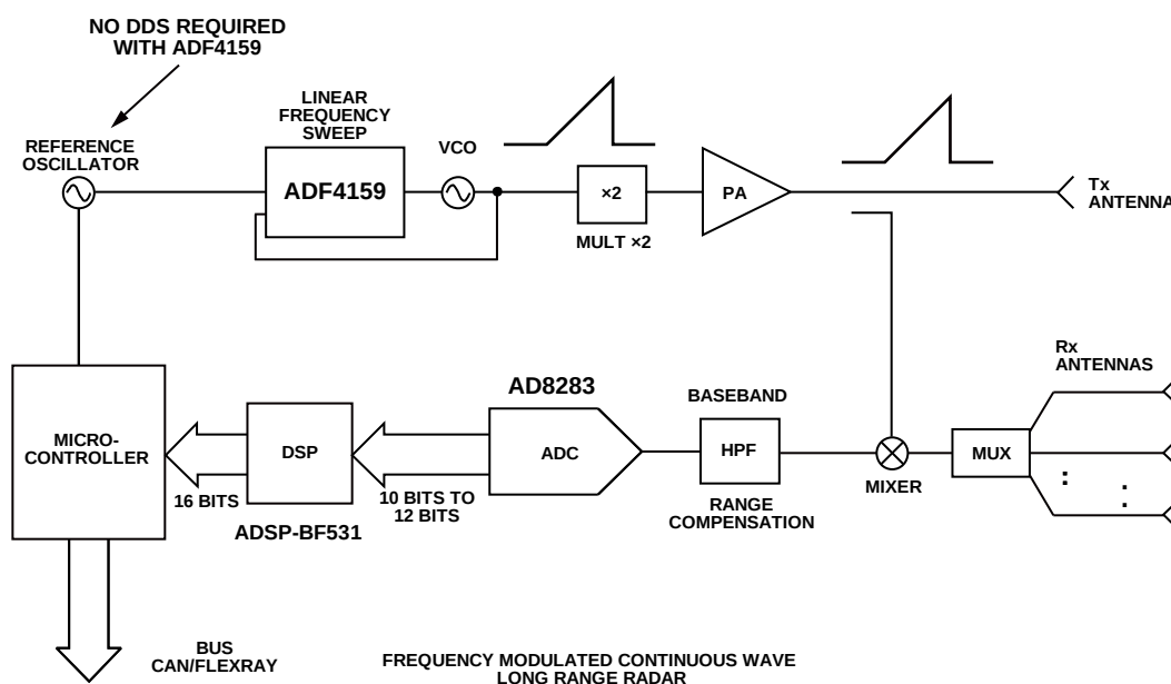
Figure 55. FMCW Radar with the ADF4159
