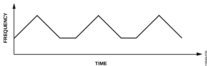
Figure 43. Delay Between Ramps for Triangular Mode
