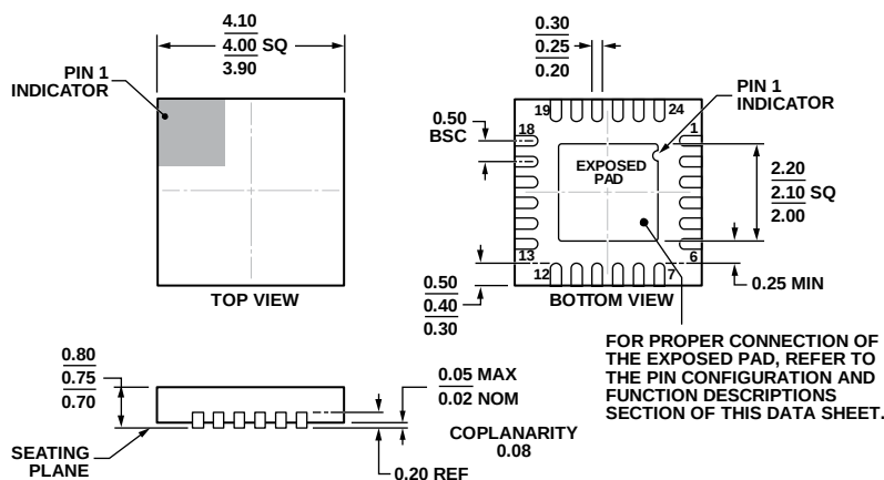
Figure 56. 24-Lead Lead Frame Chip Scale Package [LFCSP_WQ] 4 mm x 4 mm Body, Very Very Thin Quad (CP-24-10) Dimensions shown in millimeters
