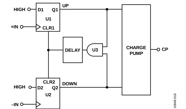
Figure 21. PFD Simplified Schematic
