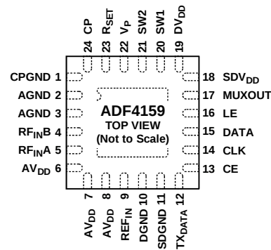
Figure 5. Pin Configuration
