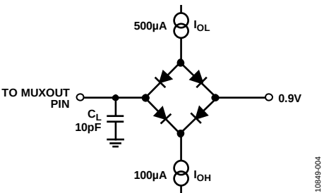
Figure 4. Load Circuit for MUXOUT Timing, C L = 10 pF
