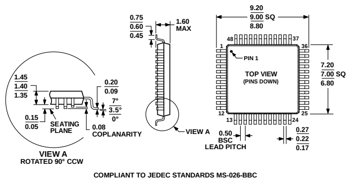
Figure 40. 48-Lead Low-Profile Quad Flat Package [LQFP] (ST-48) Dimensions shown in millimeters
