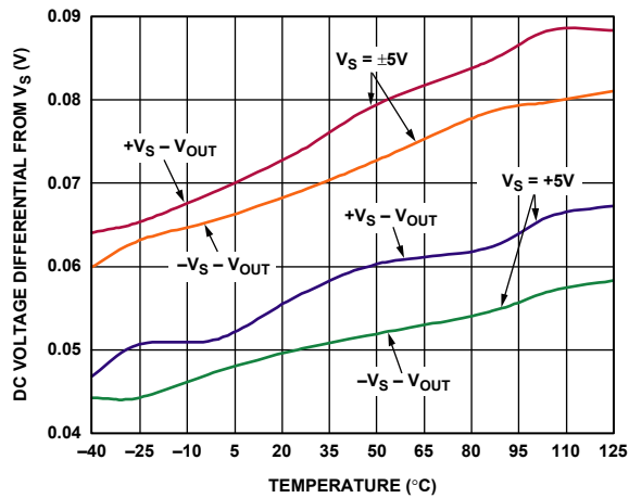
Figure 31. Output Saturation vs. Temperature for Various Supplies
