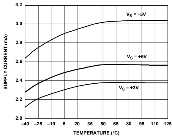
Figure 32. Supply Current vs. Temperature for Various Supplies
