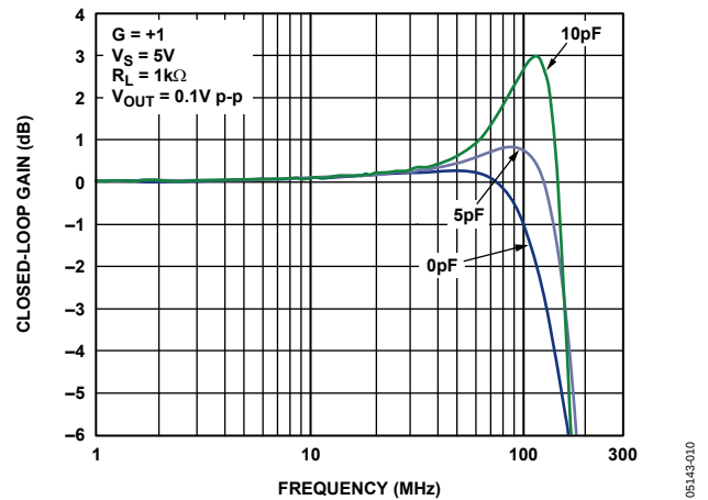
Figure 9. Small-Signal Frequency Response for Various Capacitive Loads
