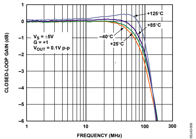
Figure 10. Small-Signal Frequency Response for Various Temperatures
