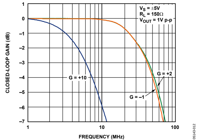
Figure 11. Large-Signal Frequency Response for Various Gains
