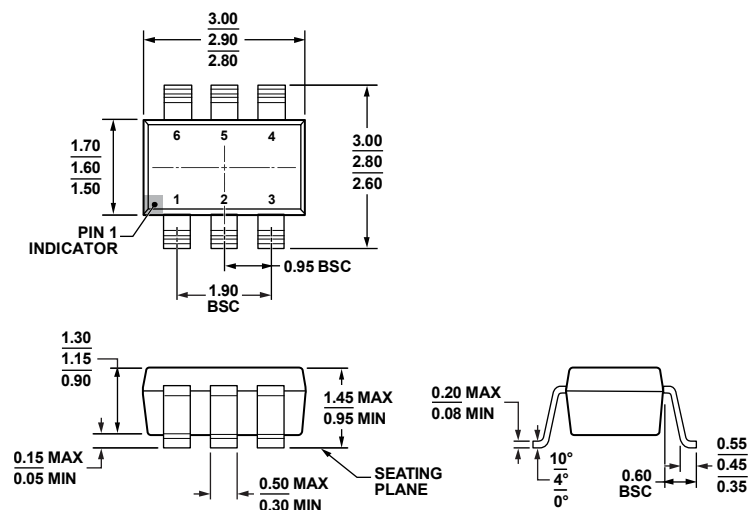
Figure 48. 6-Lead Small Outline Transistor Package [SOT-23] (RJ-6)
