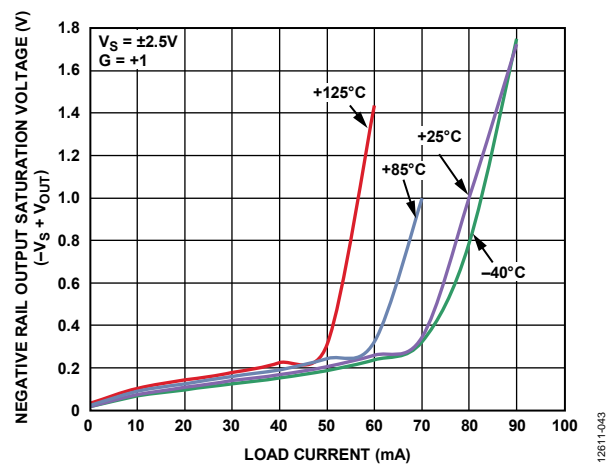
Figure 56. Negative Rail Output Saturation Voltage ( -V_S + V_{OUT} ) vs. Load Current for Various Temperatures
