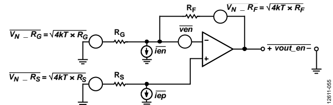
Figure 66. Noise Sources in Typical Gain Configurations
