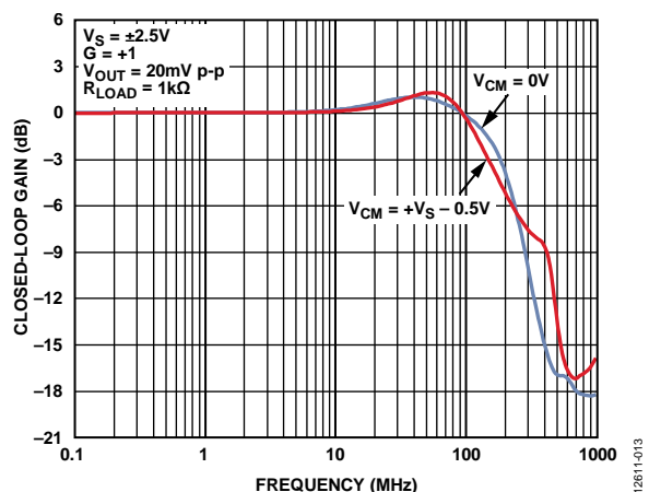
Figure 18. Small Signal Frequency Response for Various Input Common-Mode Voltages ( V_{CM} )
