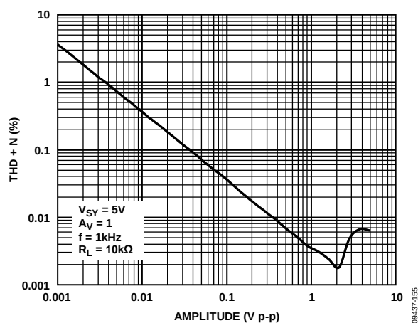
Figure 60. THD + N vs. Amplitude
