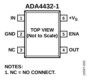
Figure 5. ADA4432-1 6-Lead SOT-23 Pin Configuration, Top View
