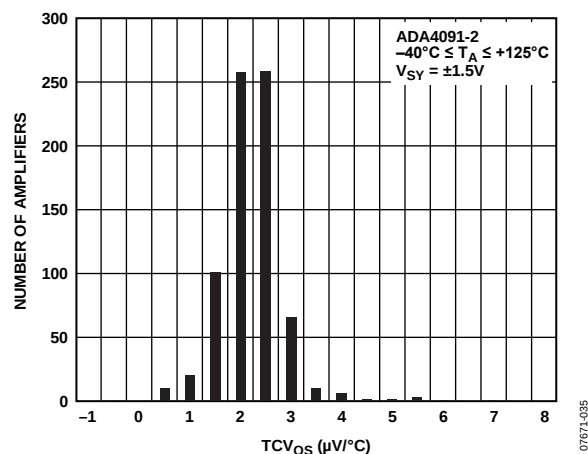
Figure 6. TCVOS Distribution
