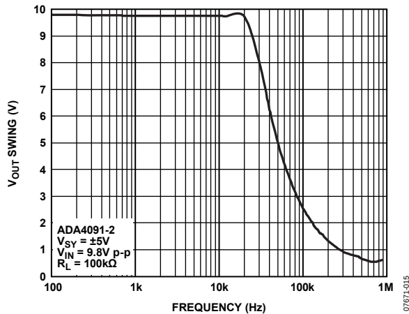
Figure 24. Output Voltage Swing vs. Frequency
