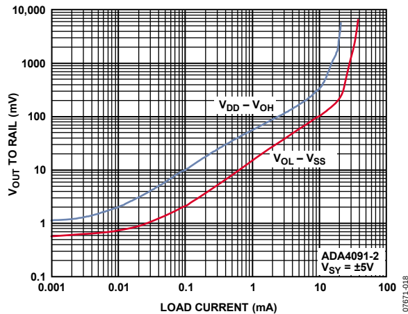
Figure 25. Dropout Voltage vs. Load Current
