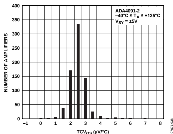
Figure 18. TCV_{OS} Distribution
