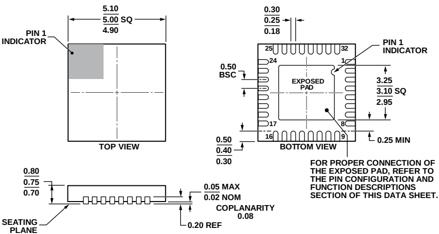
COMPLIANT TO JEDEC STANDARDS MO-220-WHHD. Figure 19. 32-Lead Lead Frame Chip Scale Package [LFCSP_WQ] 5 mm × 5 mm Body, Very Very Thin Quad (CP-32-7) Dimensions shown in millimeters
