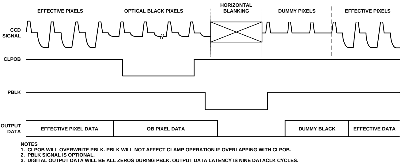
Figure 15. Typical CCD Mode Line Clamp Timing
