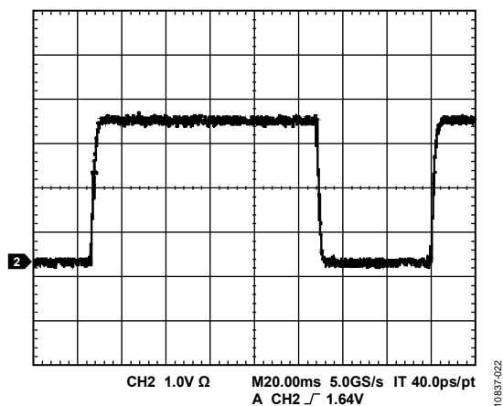
Figure 22. SYNC_OUT ( f_{\text{SYNCCLK}}/384 )
